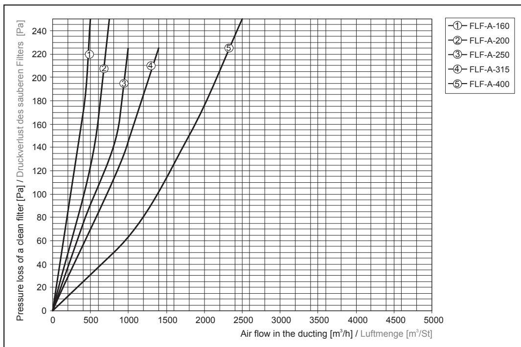
Pressure loss curves – FLF-A – filtration class ePM 1 55% (F7)
