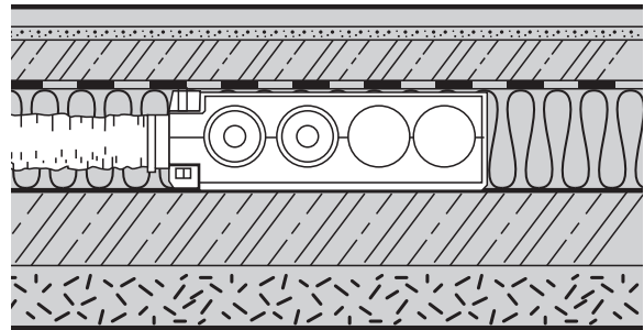
Floor installation
